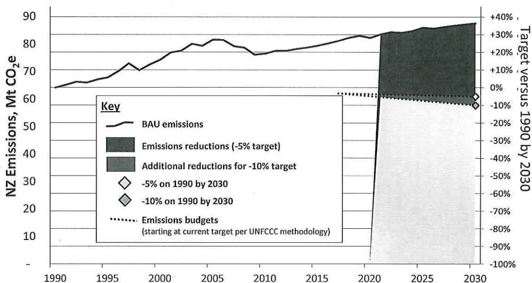
Figure 4 An illustration of the additional emissions reductions required for a target of -10% vs -5% on 1990
